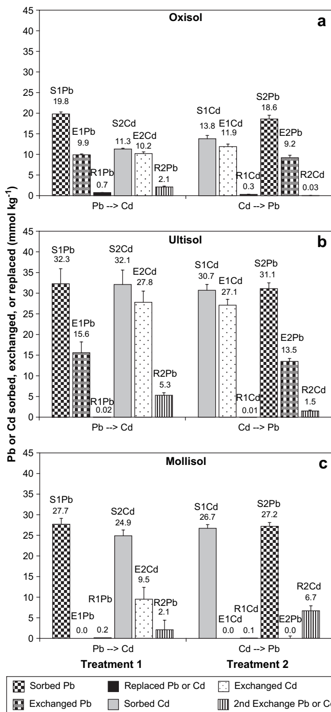
Fig. 1. Monometal sequential addition of Pb → Cd (Treatment 1) or Cd → Pb (Treatment 2) to the (a) Oxisol, (b) Ultisol, and (c) Mollisol soils. S, E, and R represent the amount of sorbed, exchanged, or replaced metal, respectively. The numbers following the letter designations indicate the order of metal addition to the soils. These designations are applicable for each of the soils in this figure.
