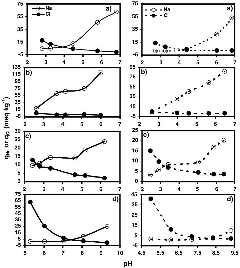
Fig. 2. AEC and CEC of an Oxisol (a), Ultisol (b), kaolinite (c) and goethite (d) as a function of pH and ionic strength. q_{Na} (measure of CEC) and q_{Cl} (measure of AEC) are absolute values of surface charge as estimated by the retention of Na^+ and Cl^- , respectively. Solid lines and dashed lines were determined in 0.01 M NaCl and 0.001 M NaCl, respectively.
